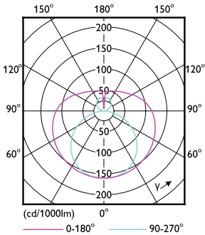
Light Distribution Diagram - CorePro LEDtube 600mm HO 8W 830 T8
